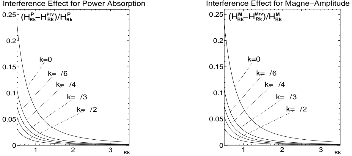
Figure 15: The rate (H_{Rk}^P - H_{Rk}^{Prv})/H_{Rk}^P of the interference effects (H_{Rk}^P - H_{Rk}^{Prv}) for the peak-height H_{Rk}^P of the power absorption P_k^{(0)}(\omega) , are displayed varying the damping constant \gamma_{Rk} of the phonon reservoir, scaled by J_1 , from 0.5 to 3.5 for the cases of wave numbers k = 0, \pi/6, \pi/4, \pi/3, \pi/2 , and for the spin-magnitude S = 5/2 , the temperature T given by k_B T/(\hbar J_1) = 1.0 and the anisotropy energy \hbar K given by K/J_1 = 2.0 , with J_2/J_1 = 1.0 and \omega_z/J_1 = 1.0 . Here, the peak-height H_{Rk}^P is the approximate formula given by (3.27), and H_{Rk}^{Prv} is the one without the corresponding interference terms X_{k1(2)}^\alpha(\omega) in the approximate formula (3.27).
