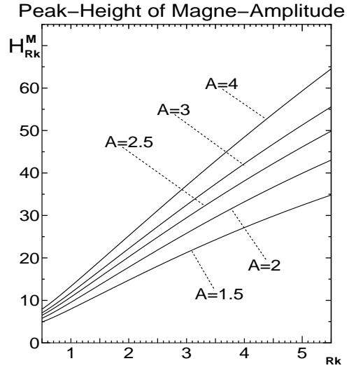
Figure 17: The approximate formula (3.27) for the peak-height H_{Rk}^P in the resonance region of the power absorption P_k^{(0)}(\omega) , scaled by \hbar^2 \gamma^3 |H_k|^2 , is displayed varying the damping constant \gamma_{Rk} of the phonon reservoir, scaled by J_1 , from 0.5 to 5.5 for the cases of anisotropy energies \hbar K given by A = K/J_1 = 1.5, 2.0, 2.5, 3.0, 4.0 , and for the temperature T given by k_B T / (\hbar J_1) = 1.0 and the spin-magnitude S = 5/2 , with J_2/J_1 = 1.0 and \omega_z/J_1 = 1.0 .
